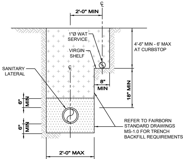
BENCHED UTILITY TRENCH - SECTION A-A
