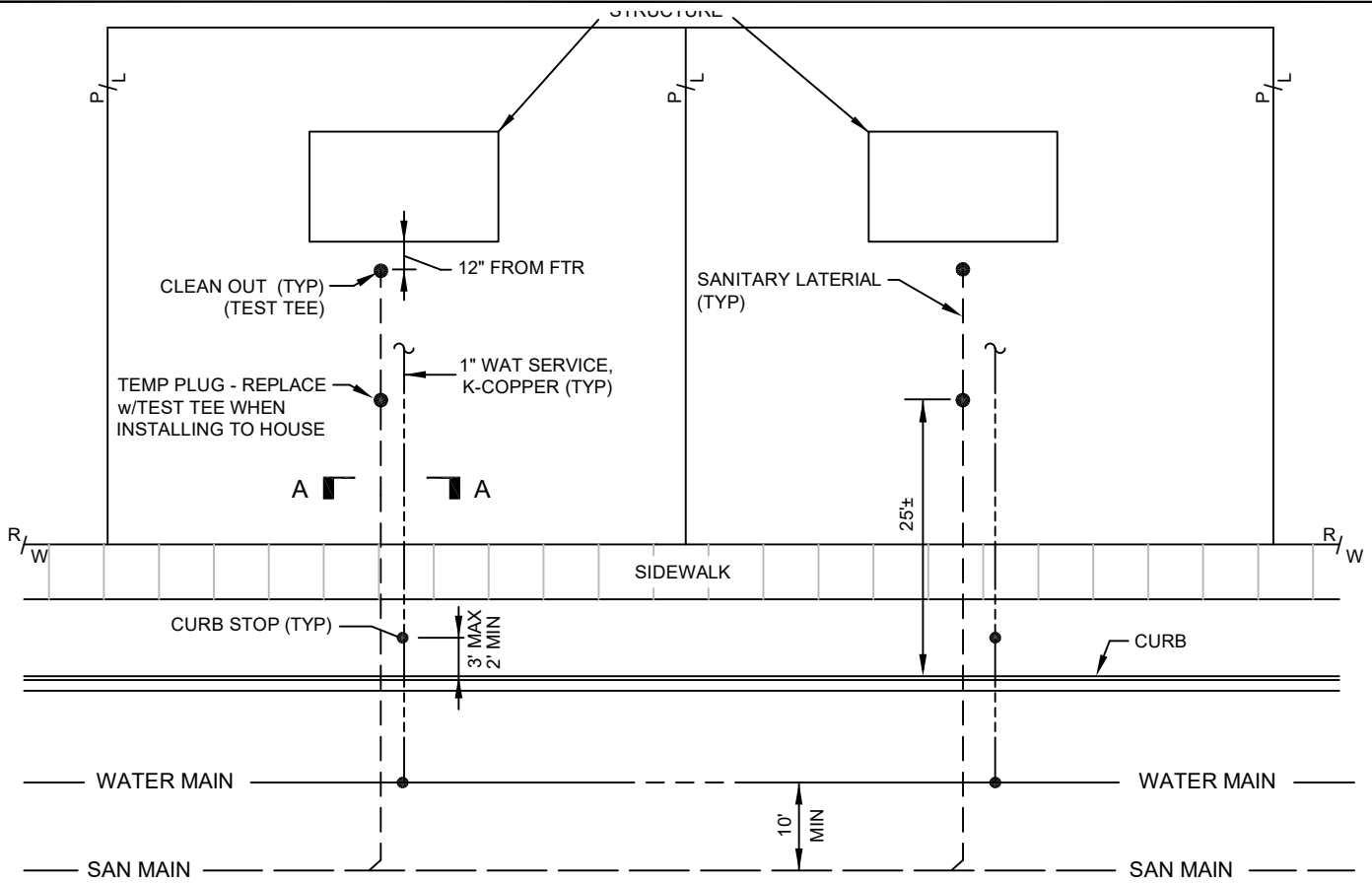
SERVICE UTILITY LAYOUT PLAN
