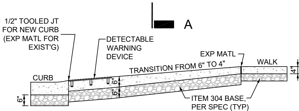
RAMP SECTION A-A
