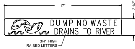
LOGO DETAIL SCALE 1:4
